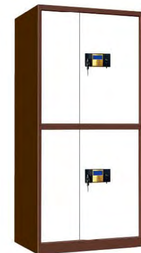
SW-B079 电子码通双节柜 Electronic Lock Cabinet H1850 × W900 × D430mm
